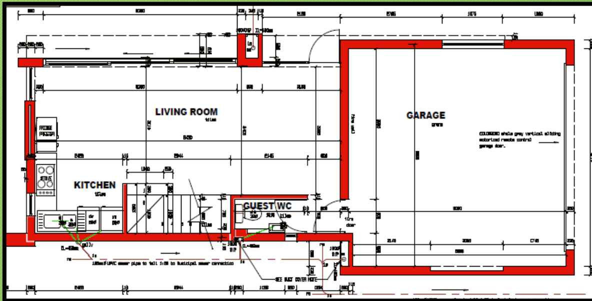
GROUND FLOOR PLAN UNIT 2 & 11
