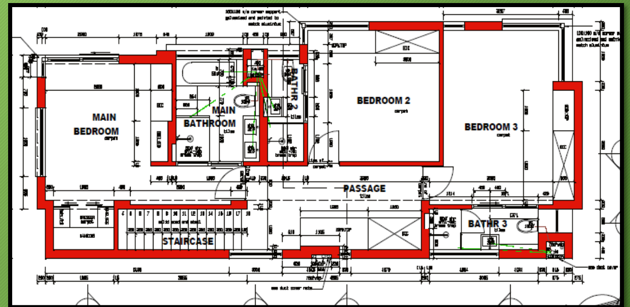
FIRST FLOOR PLAN UNIT 4 - 10
