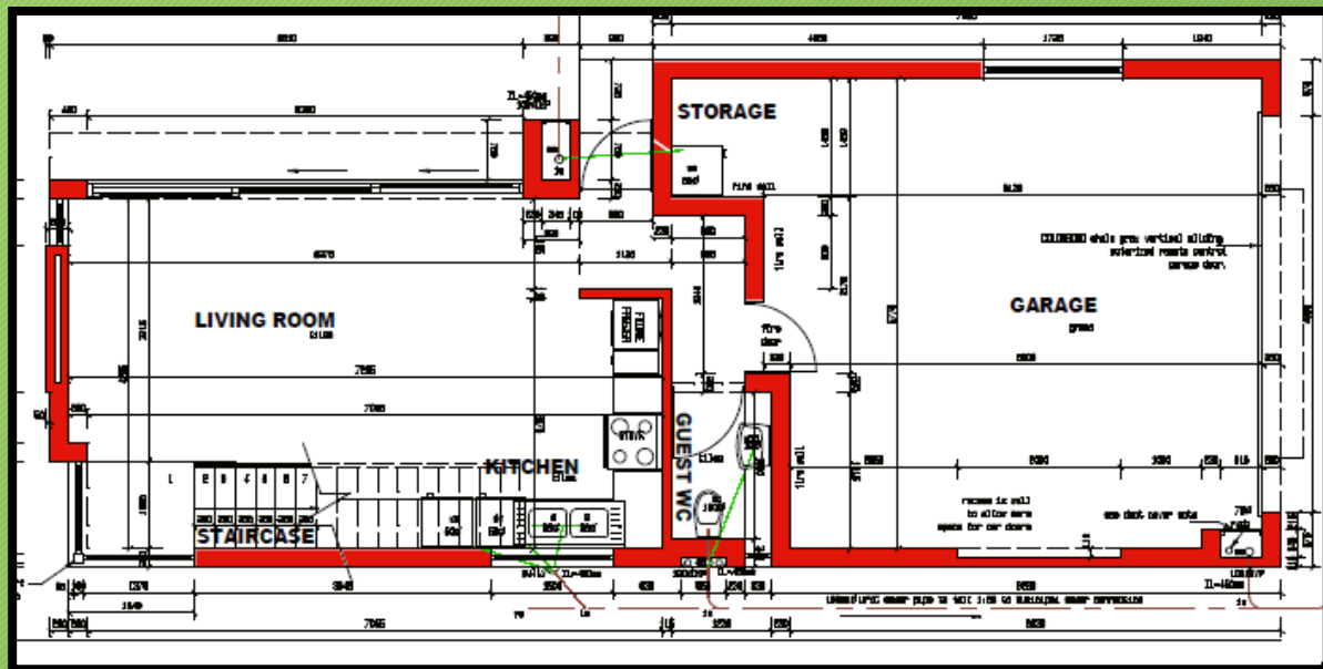
GROUND FLOOR PLAN UNIT 4 - 10
