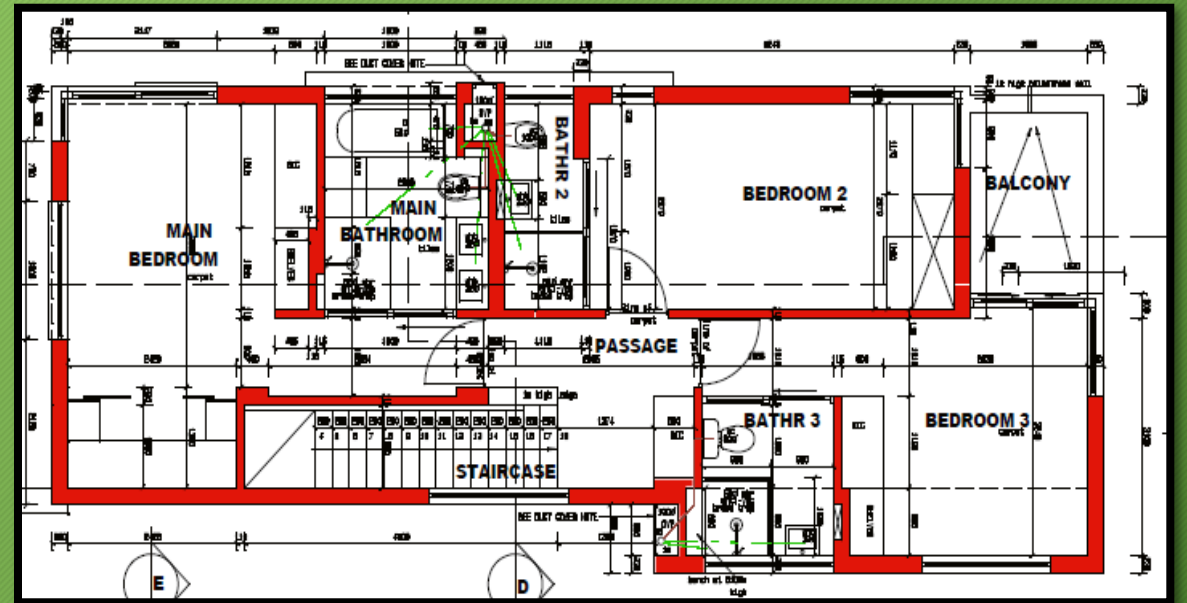
FIRST FLOOR PLAN UNIT 2 & 11
